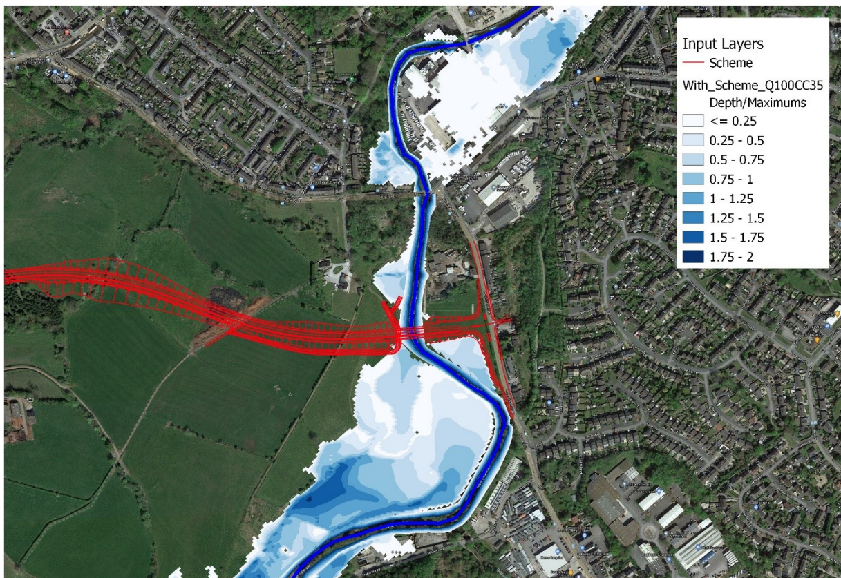
Insert 4-6 Post Scheme Flood depth map for the 1% AEP event plus 35% climate change allowance
